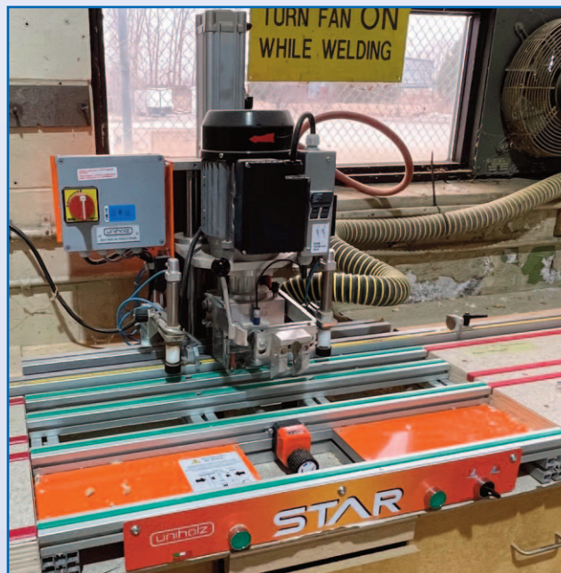
UNIHOZL STAR HINGE BORING MACHINE
