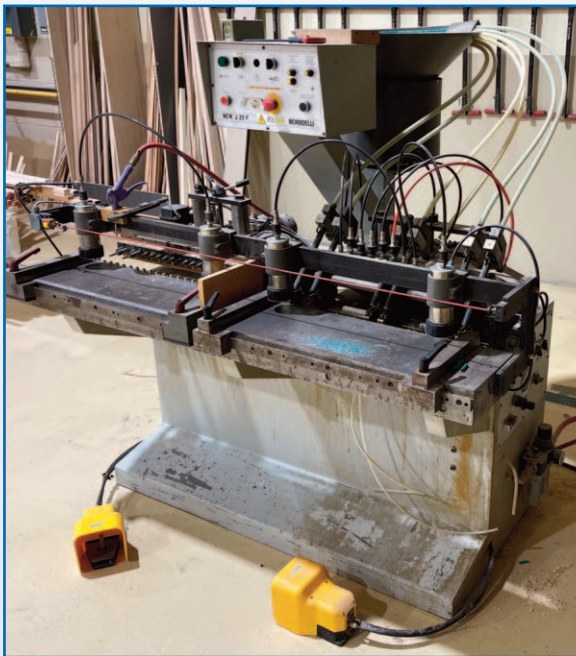
MORBIDELLI N/J20F DOWEL INSERTER
