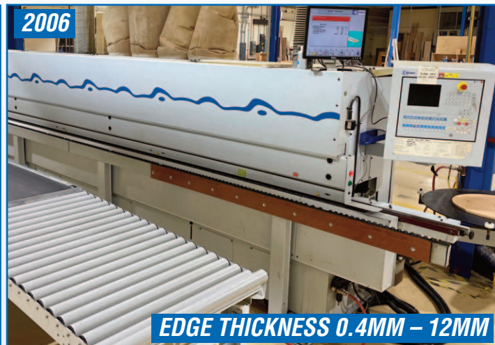
BRANDT CNC KDF 790 PROFILINE SINGLE EDGE BANDER
