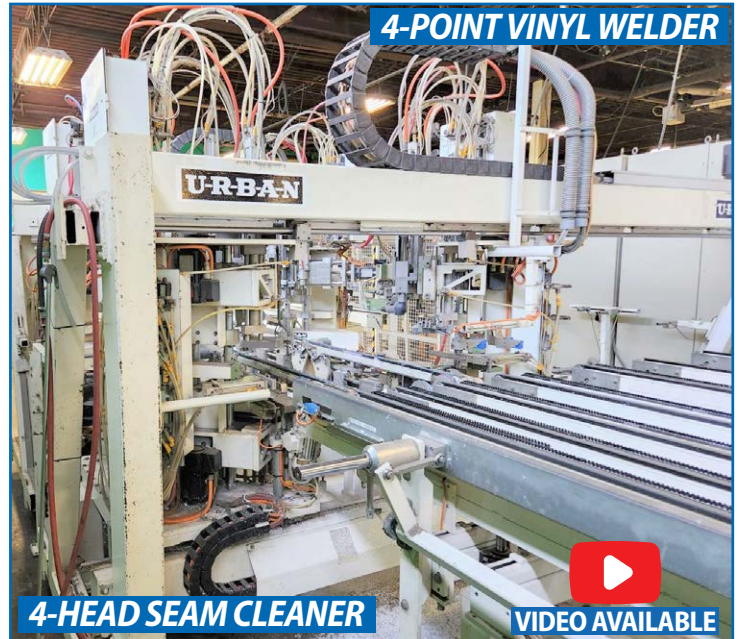
URBAN PVC PRODUCTION LINE
